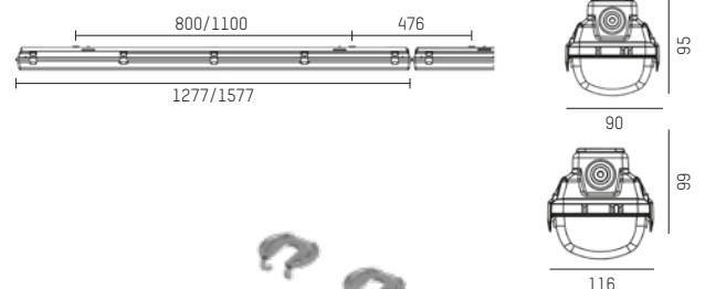
Hooks for suspension 175-013 (to be ordered separately)
